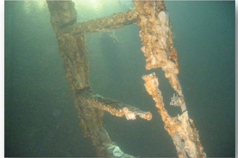
Corroded ladder structures
